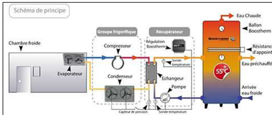
Installation BOOSTHERM
