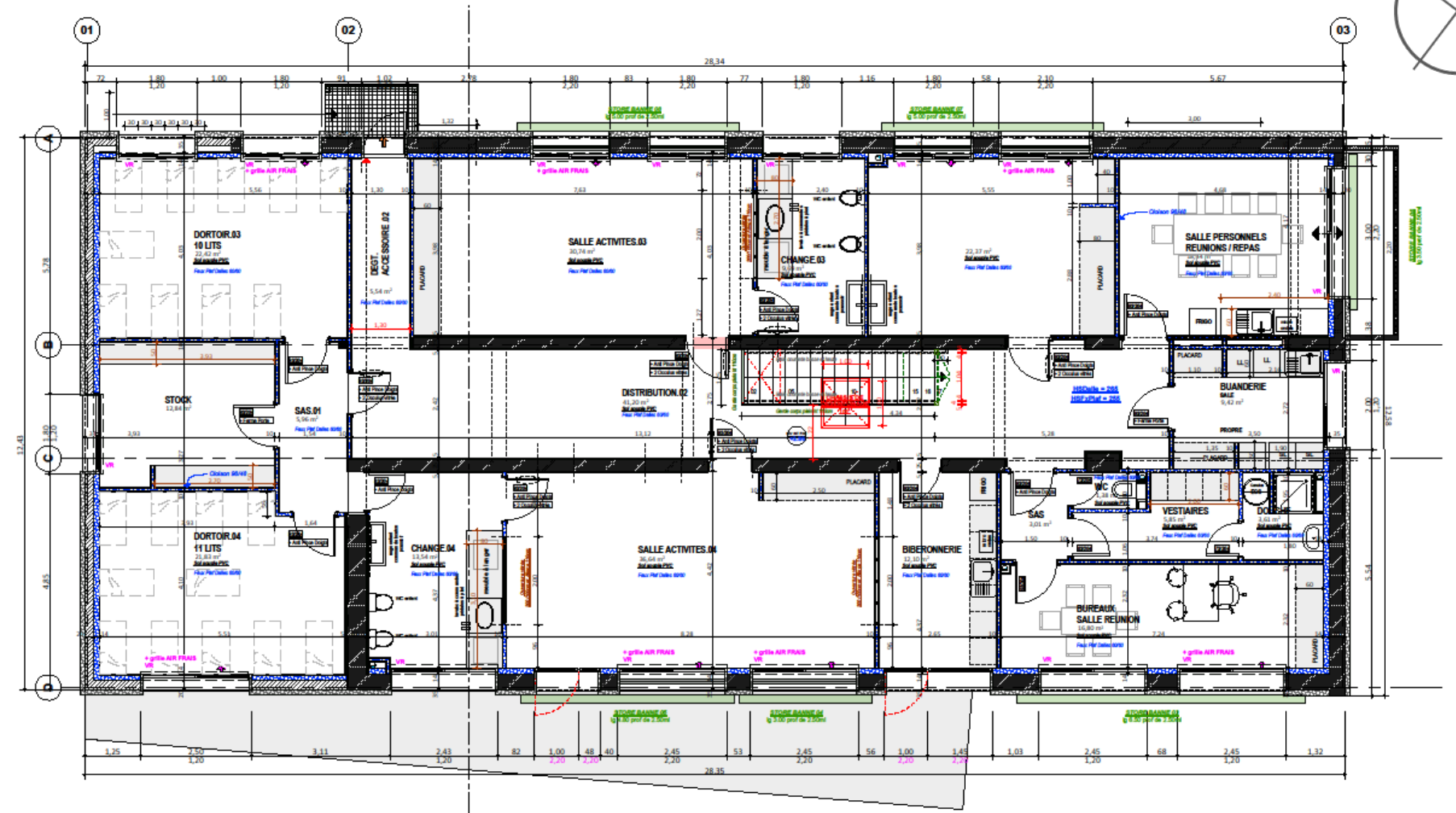
PLAN R+1 - PROJET SURFACE HABITABLE R+1: 284.68m²
